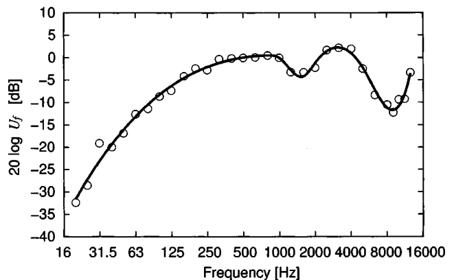
FIG. 8. U_f , a parameter in Eq. (6), reestimated using the interpolated \alpha_f shown in Fig. 7 as a solid line. Values of U_f 's are transformed into dB to show the plots in the figure. Solid line shows a smoothed line generated by a cubic B-spline function.
