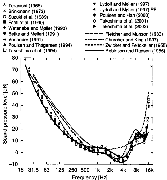
FIG. 3. Thresholds of hearing for pure tones. The four lines represent the threshold curve reported by Fletcher and Munson (1933), by Churcher and King (1937), by Zwicker and Feldtkeller (1955), and by Robinson and Dadson (1956). In the legend, PF means that the study was carried out under pressure-field listening condition.
