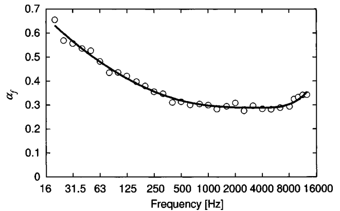
FIG. 7. Estimated \alpha_f 's from the nonlinear least squares method. Solid line shows a smoothed line generated by a cubic B-spline function.
